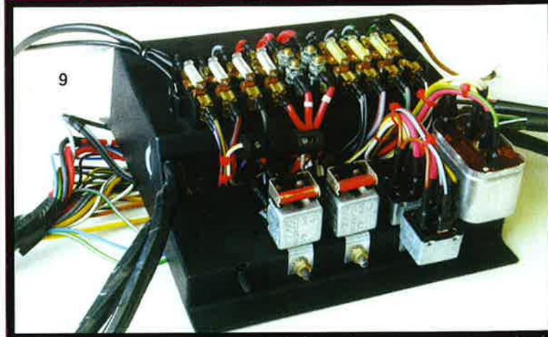
Anschaltkasten generalüberholt terminal box completely overhauled
