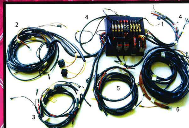
Komplettkabelbaum (ohne Instrumente) complete wiring harness (without instruments)
